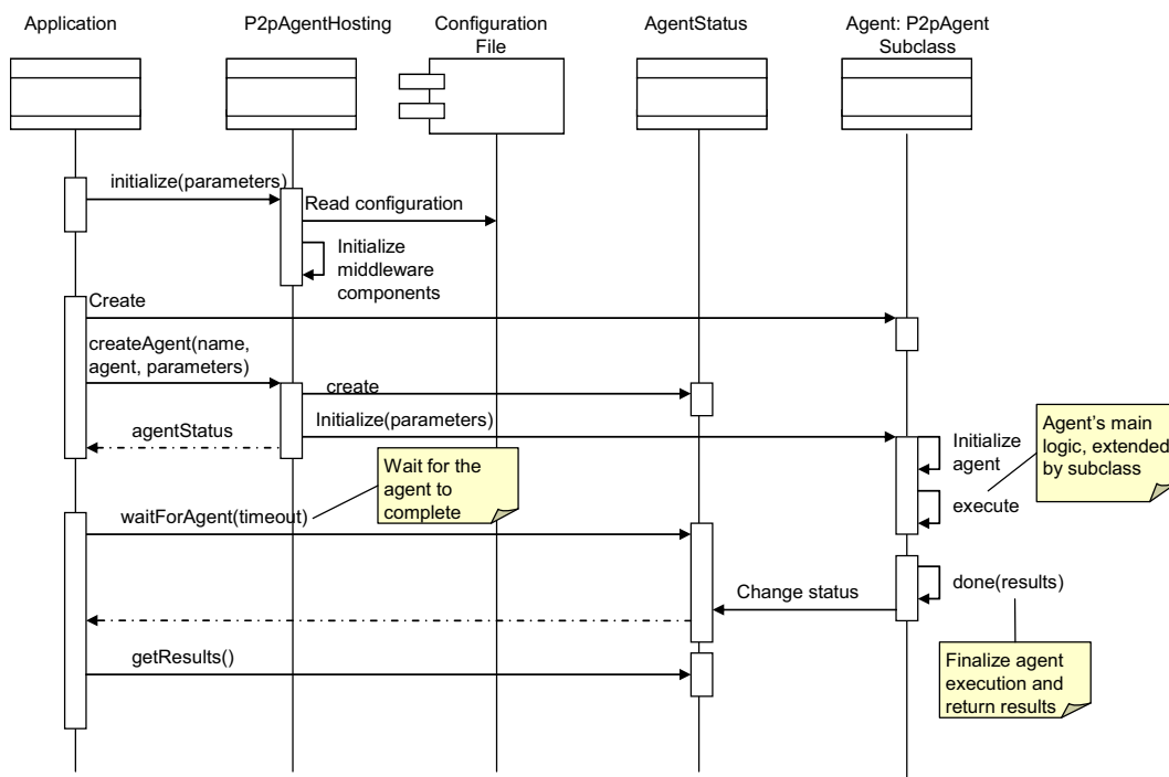
Figure 5-6 Programming model
