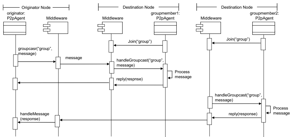
Figure 5-8 - Groupcast model
